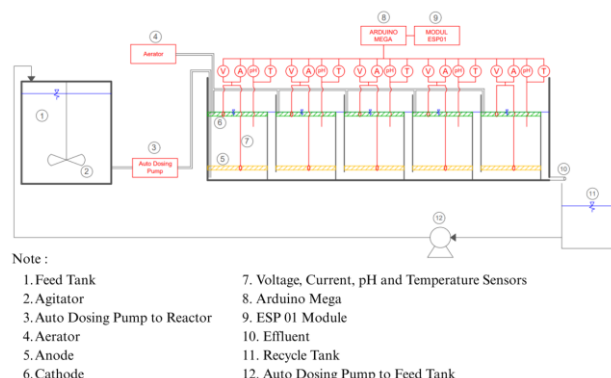
Figure 1 Design of Reactor
