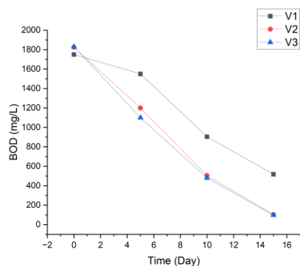
Figure 5 BOD vs Time
