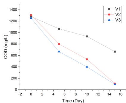
Figure 6 COD vs Time
