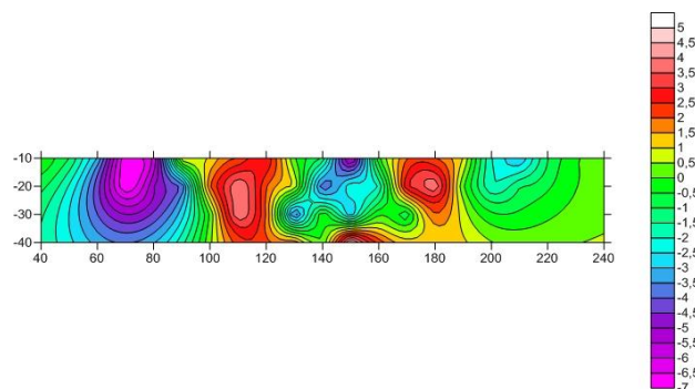
Gambar 4. Hasil filter Karous-Hjelt
