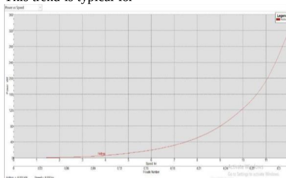
Figure 3. Power vs Speed in Maxsurf Resistance
