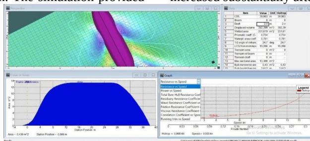
Figure 2. Resistance Analysis
