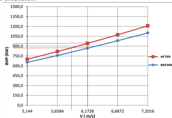
Figure 6. Speed vs Brake Horsepower (BHP) Graph
