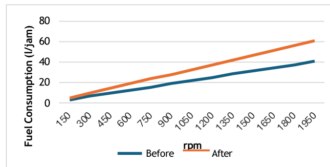
Figure 8. Relationship Between Speed and Fuel Consumption Source: data processing
