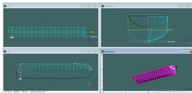
Figure 1. Ship Design in Maxsurf Modeler
