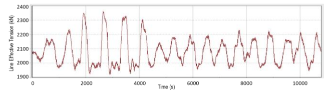
Figure 16. Effective tension on line-9 due to wave H_s = 4.5 m and direction 90° for operation scenario of the 1 st condition
