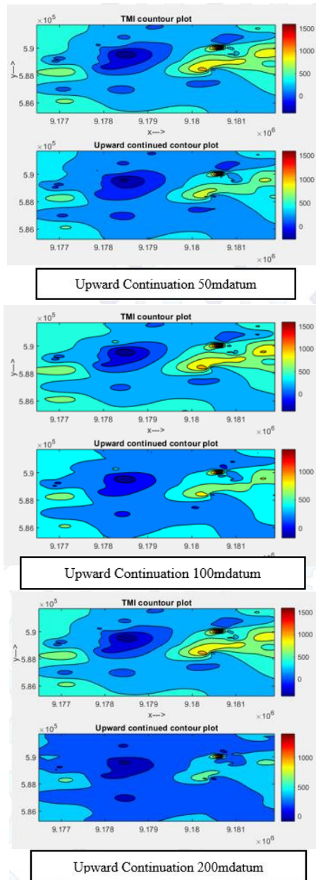
Fig 4. Comparison of datums in the Upward Continuation filter
