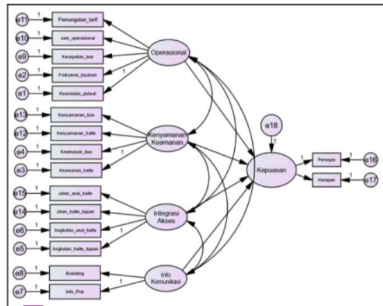
Ga 21 1. Path Analysis
