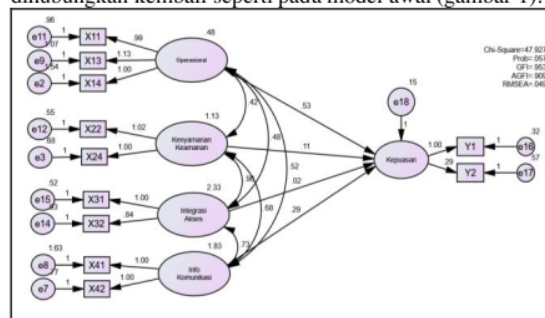
Gambar 3. Model Akhir SEM
