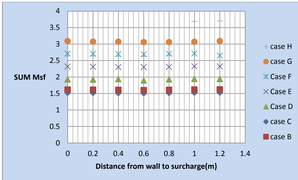
Figure 5. SUM Msf for wall depth(ULS) with distance from wall to surcharge
