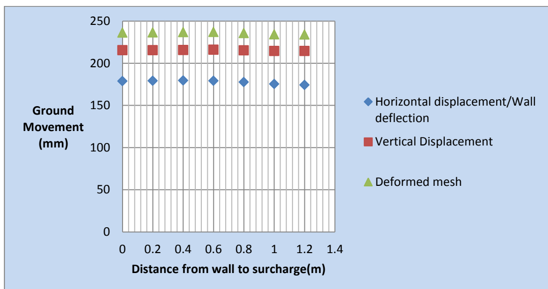
Figure 3. Ground movement with distance from wall to surcharge
