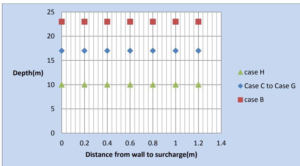
figure 4. Wall depth with distance from wall to surcharge(ULS)
