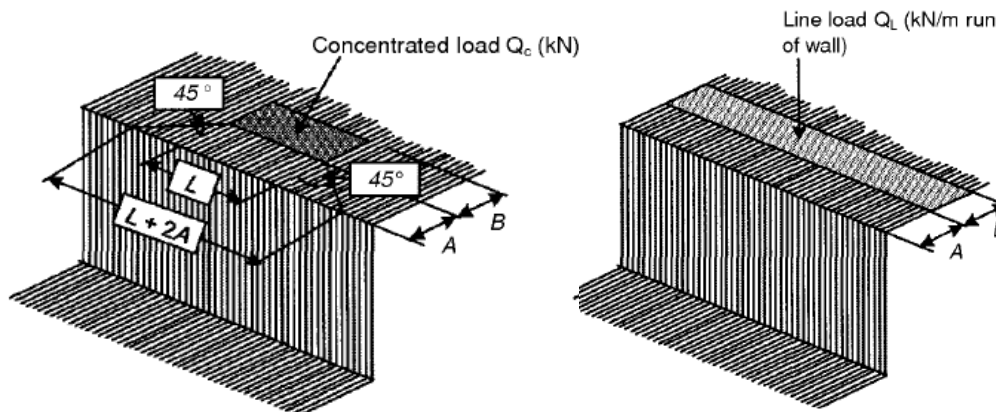
Figure 1. Concentrated and line load surcharges
