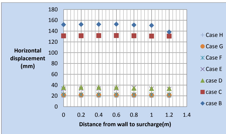
Figure 6. Horizontal displacement with distance from wall to surcharge
