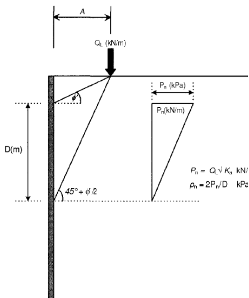
Figure 2. Pressure Diagram Line Load
